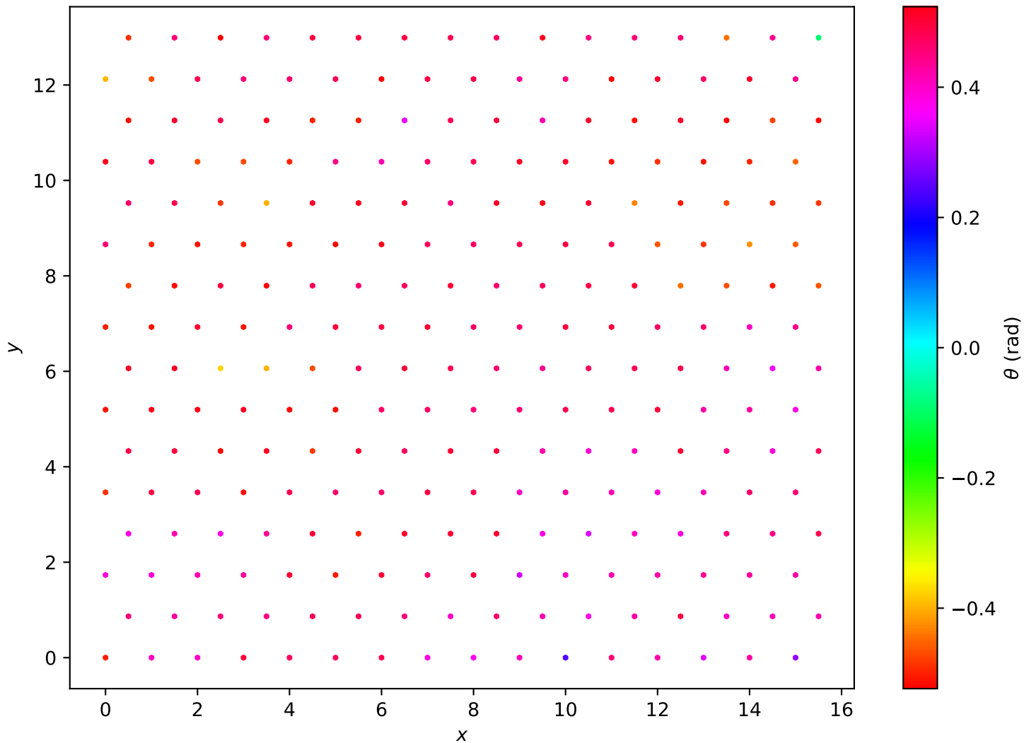
Hexagonal Lattice L=16 , T = 1.00e - 01
