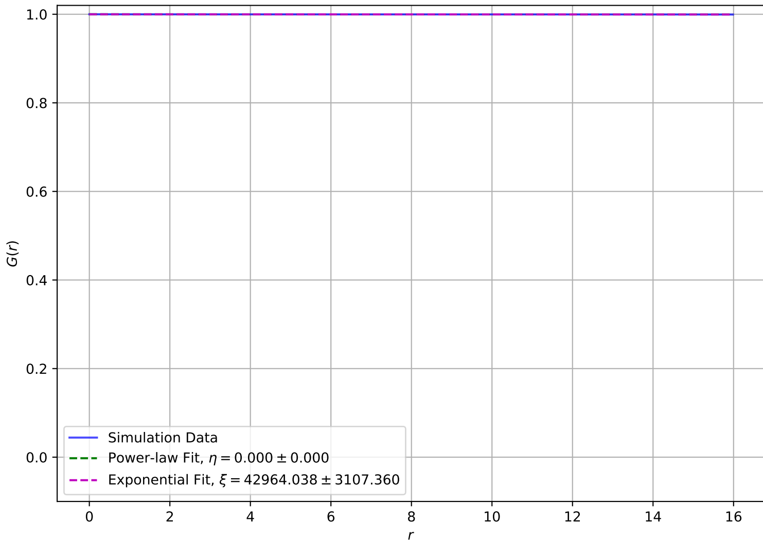
Correlation Function at T = 1.00\text{e} - 02 , L = 16
