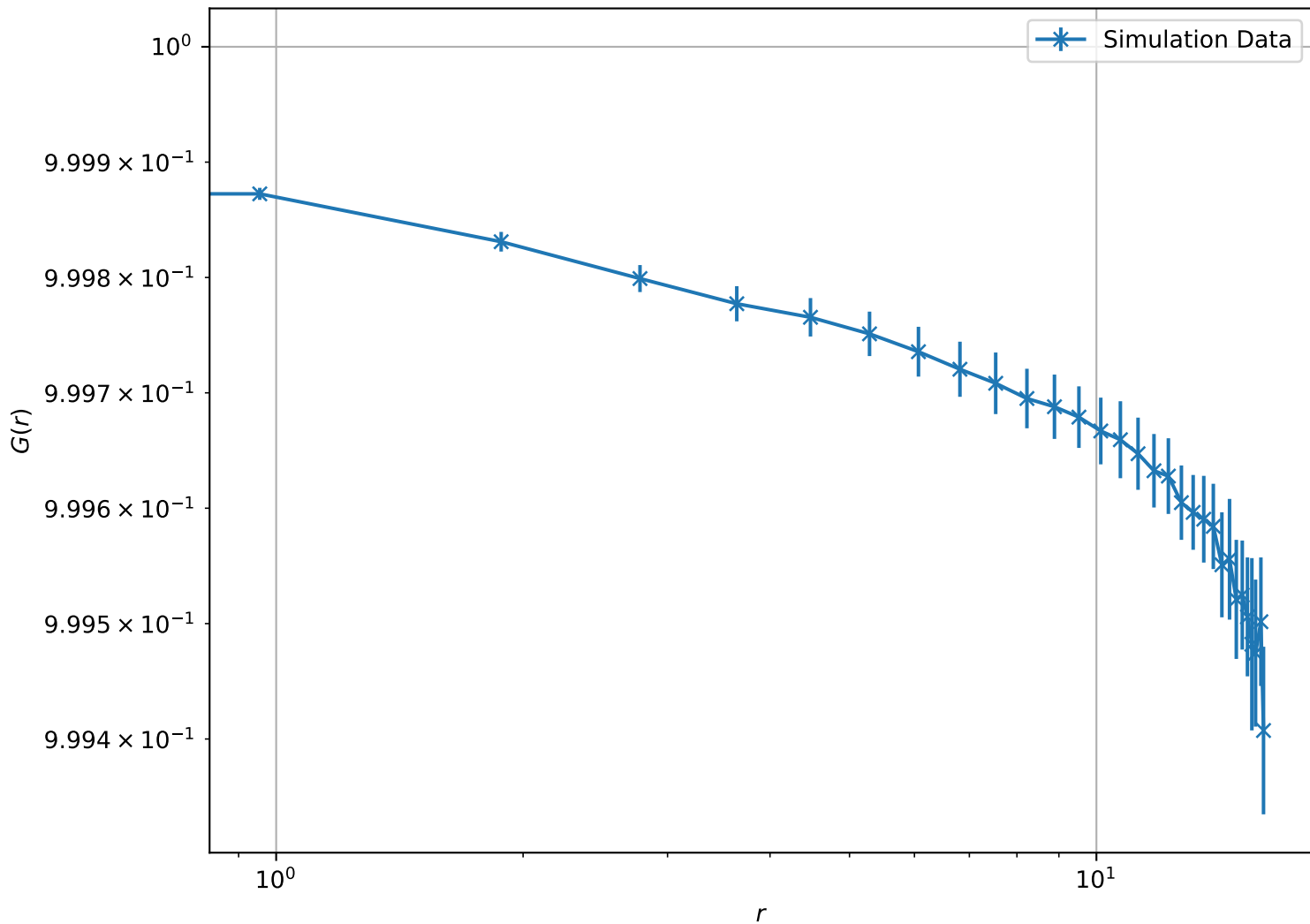
Correlation Function at T = 1.00e - 02 , L = 16 (Log-Log Scale)
