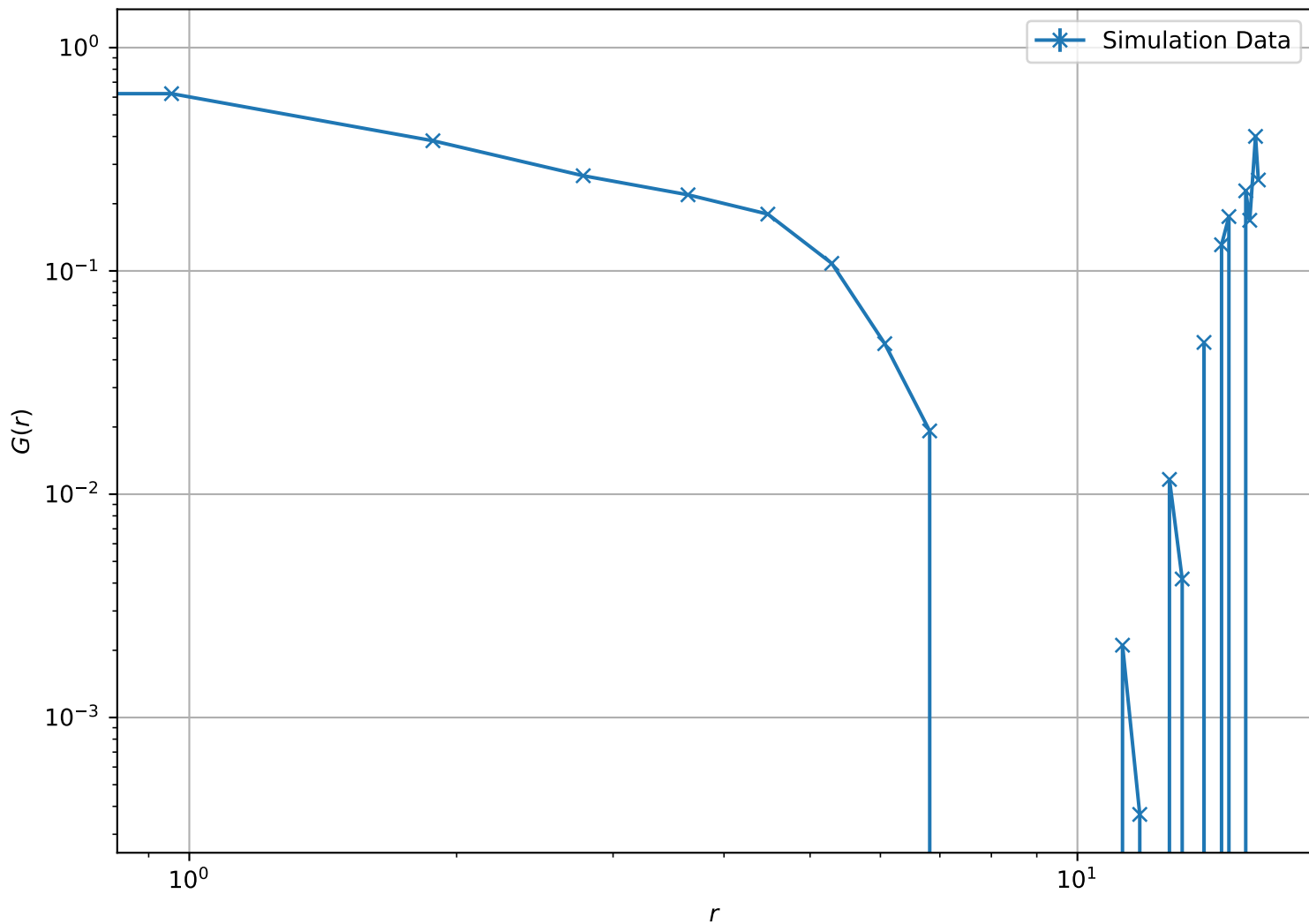
Correlation Function at T = 1.00e - 05 , L = 16 (Log-Log Scale)
