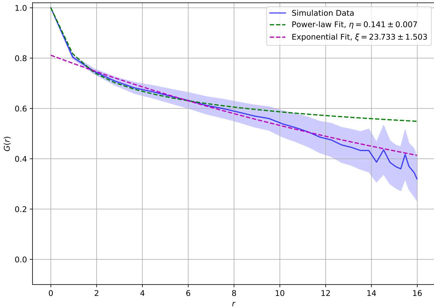
Correlation Function at T = 1.50e - 01 , L = 16
