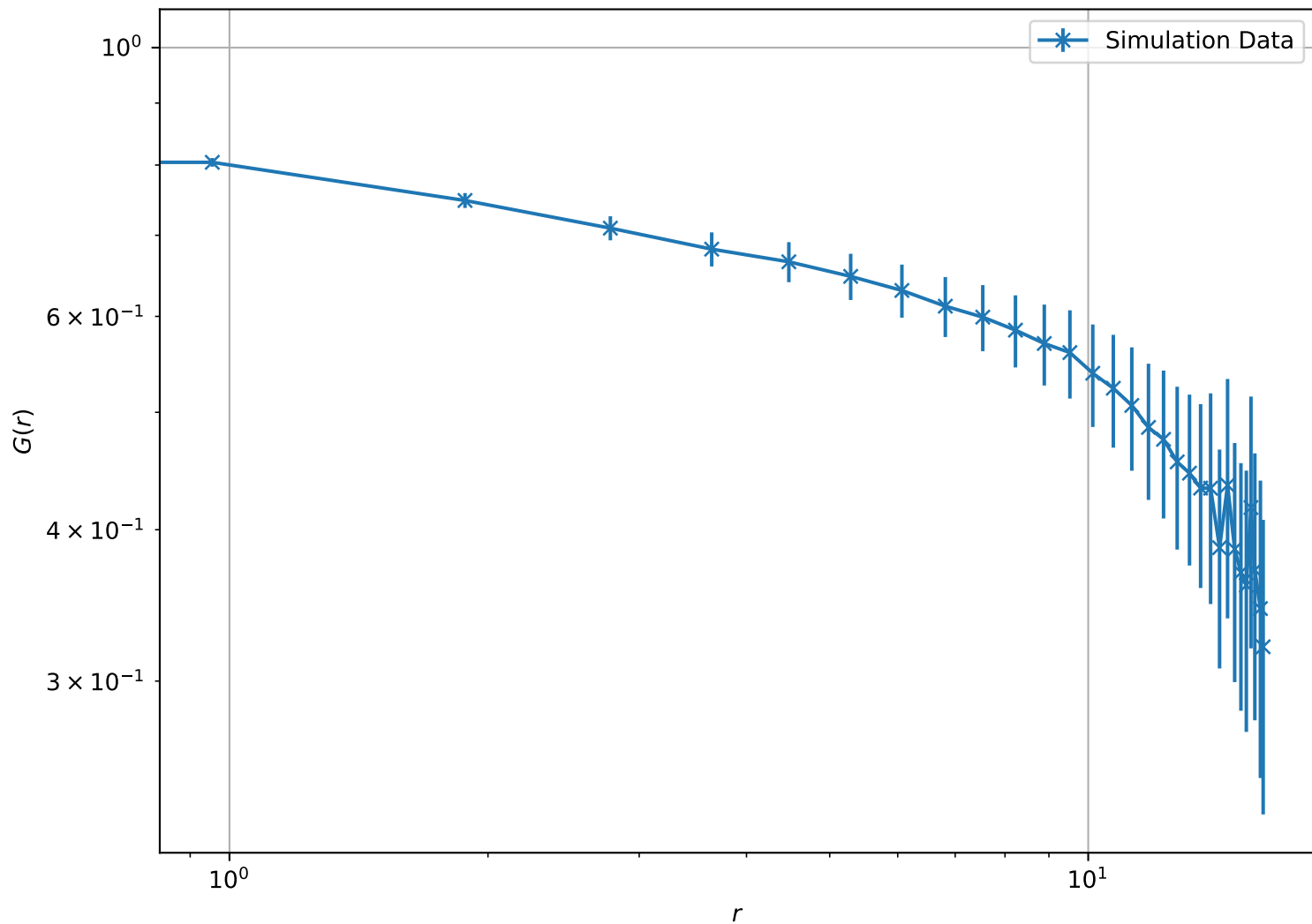
Correlation Function at T = 1.50e - 01 , L = 16 (Log-Log Scale)
