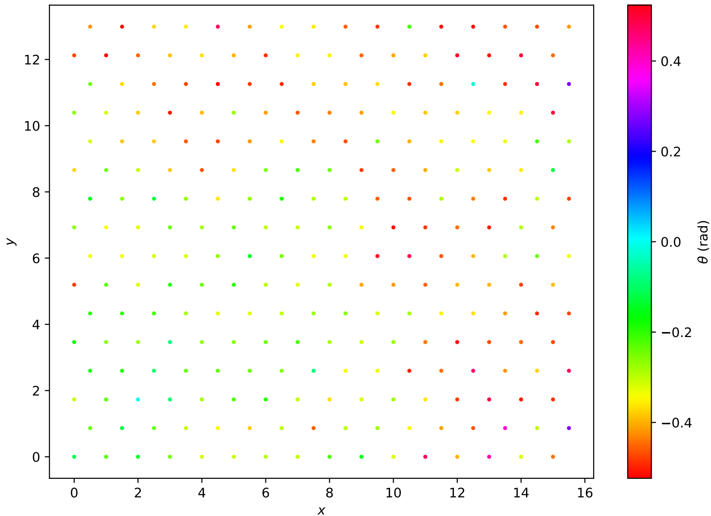
Hexagonal Lattice L=16 , T = 1.50e - 01
