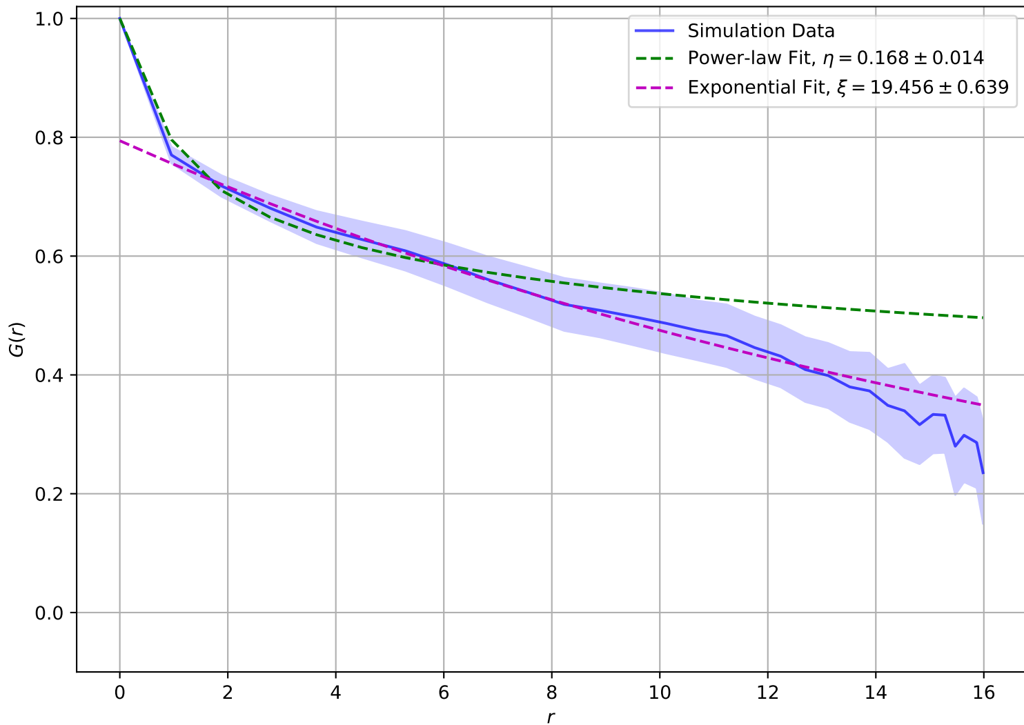
Correlation Function at T = 1.60e - 01 , L = 16
