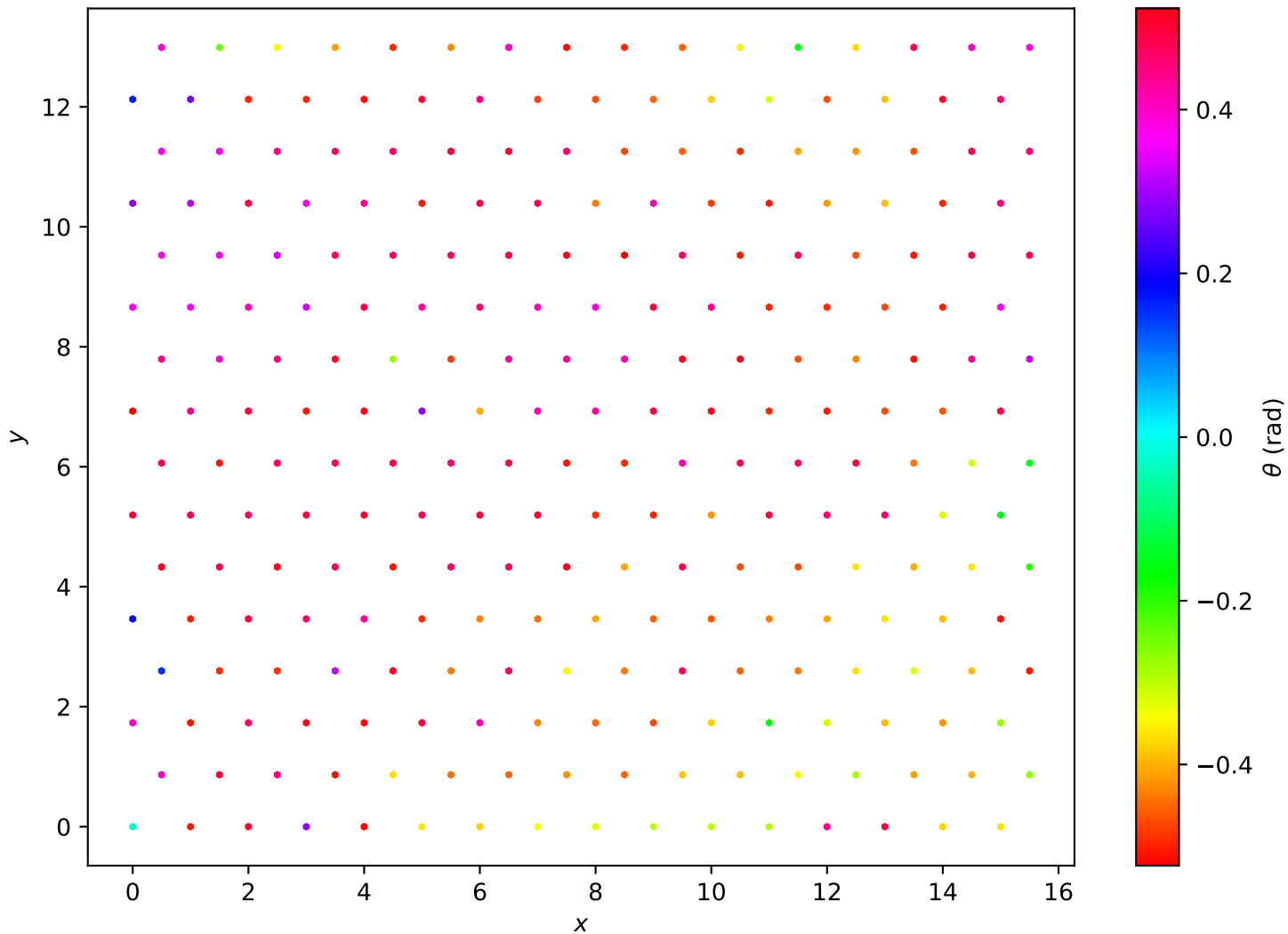
Hexagonal Lattice L=16 , T = 1.60e - 01
