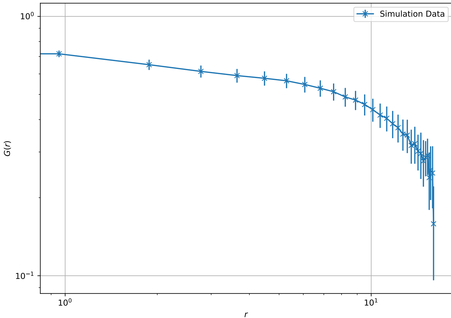
Correlation Function at T = 1.70e - 01 , L = 16 (Log-Log Scale)
