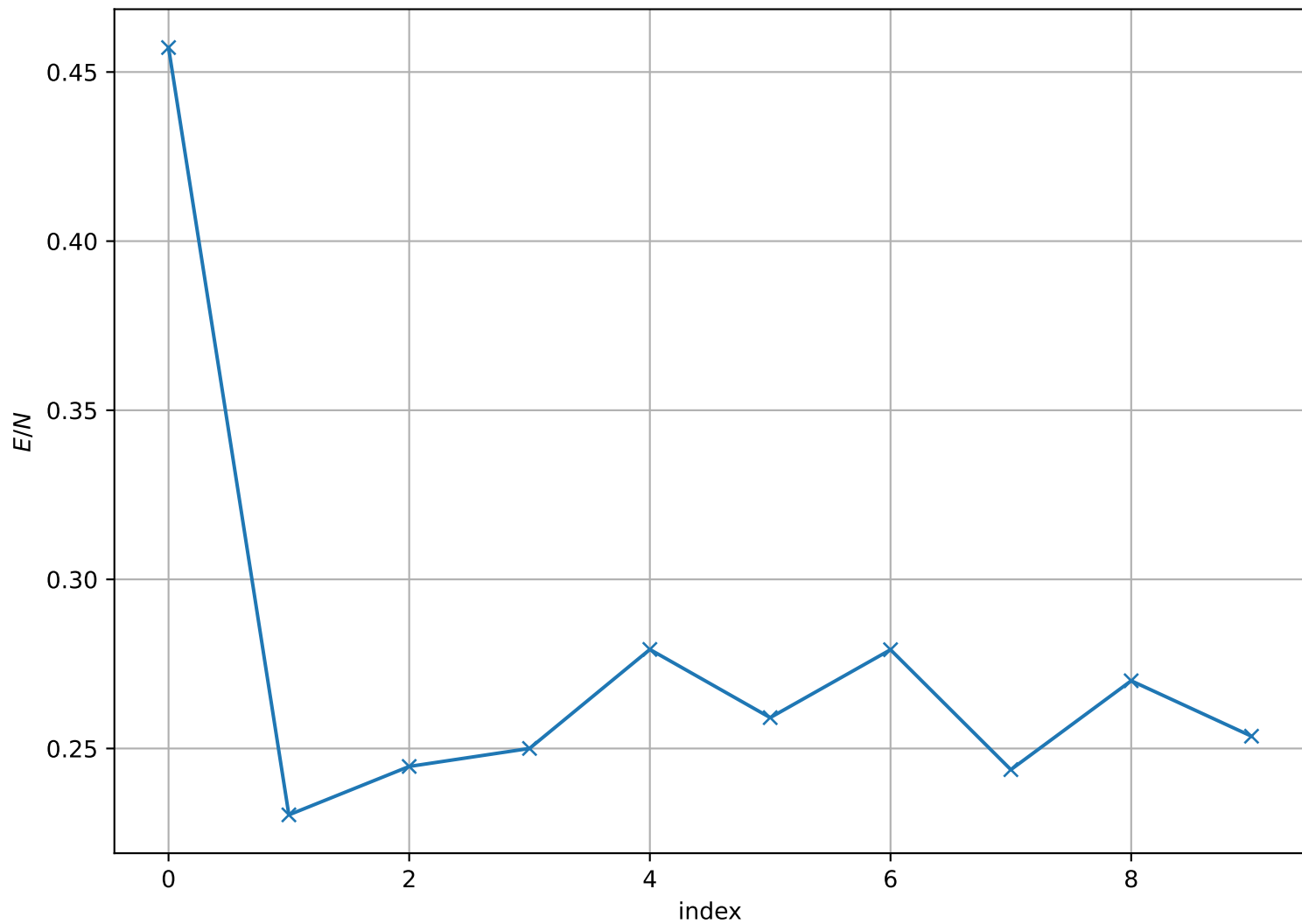
Energy per Site at T = 1.700e - 01 , L = 16
