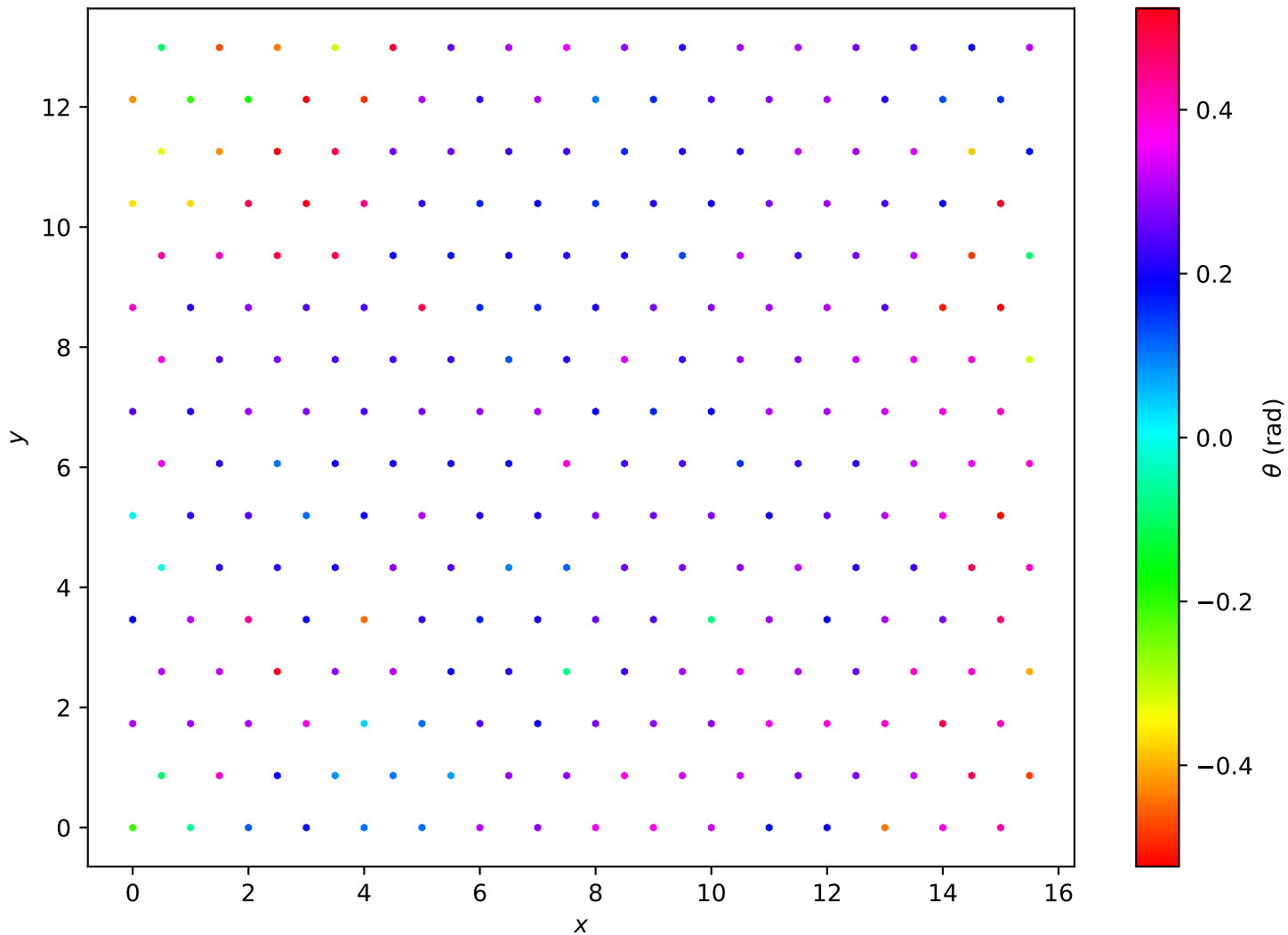
Hexagonal Lattice L=16 , T = 1.70e - 01
