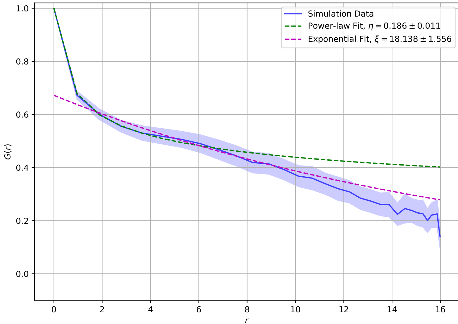
Correlation Function at T = 1.80e - 01 , L = 16
