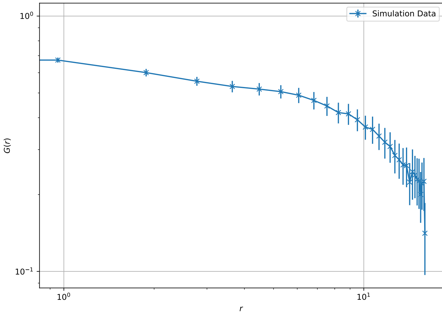
Correlation Function at T = 1.80e - 01 , L = 16 (Log-Log Scale)
