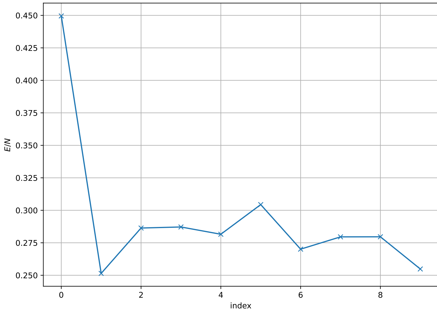
Energy per Site at T = 1.800e - 01 , L = 16
