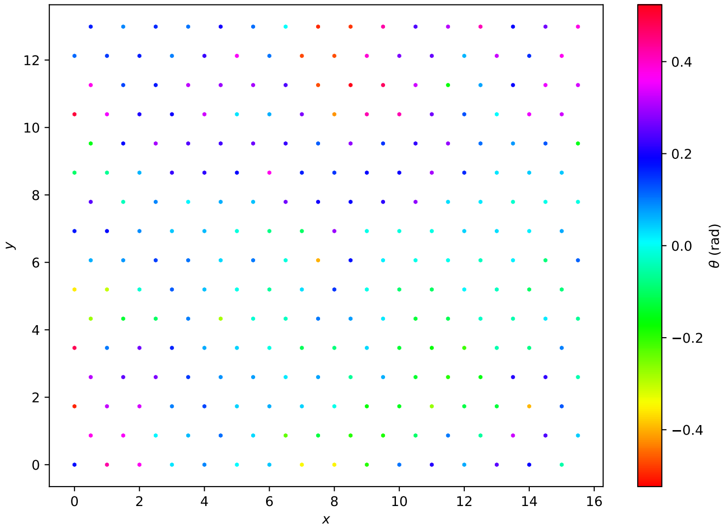
Hexagonal Lattice L=16 , T = 1.80e - 01
