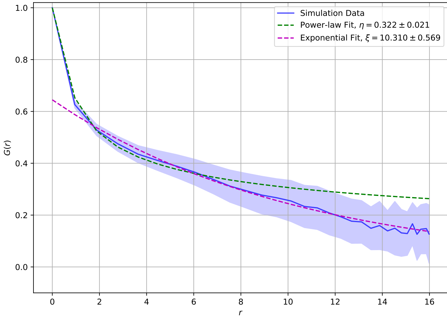
Correlation Function at T = 1.85e - 01 , L = 16
