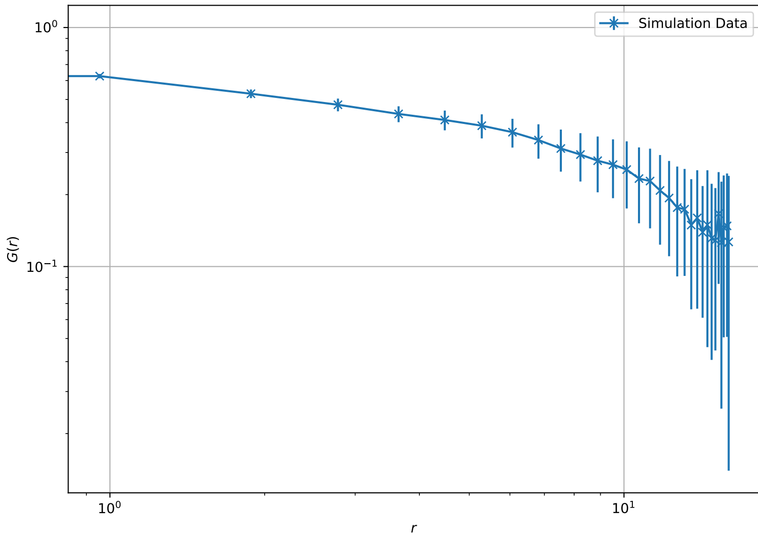
Correlation Function at T = 1.85e - 01 , L = 16 (Log-Log Scale)
