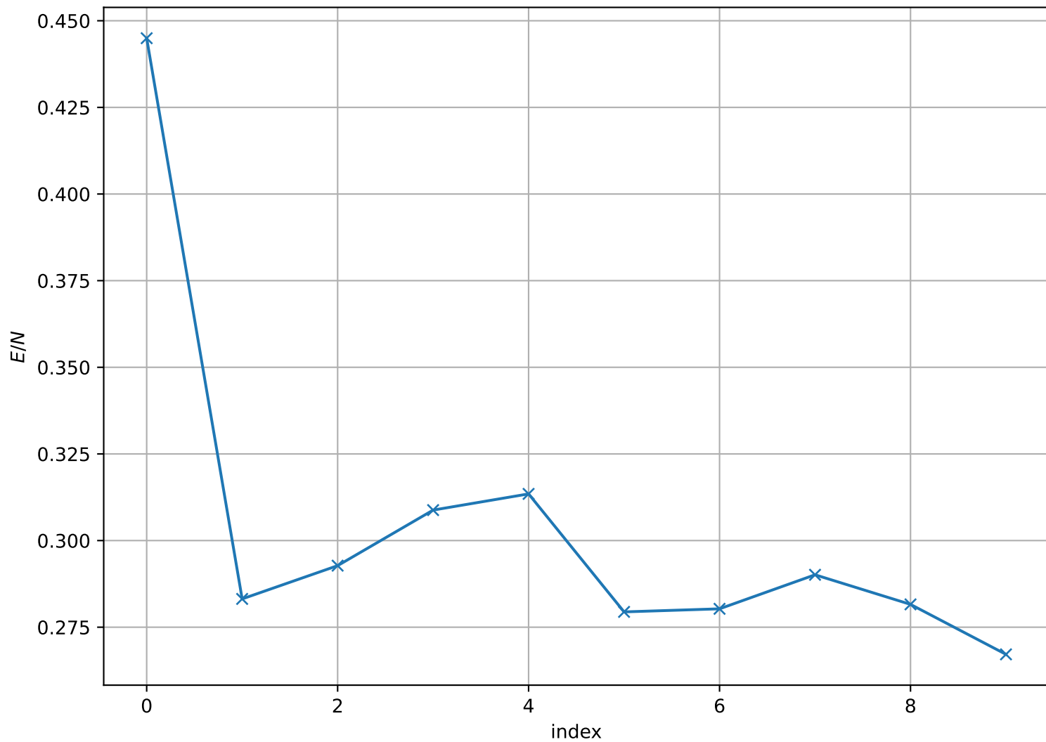
Energy per Site at T = 1.850e - 01 , L = 16
