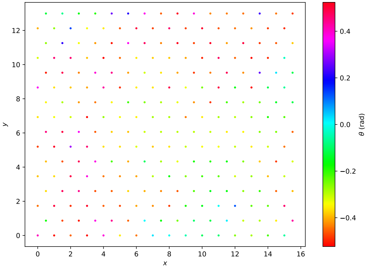
Hexagonal Lattice L=16 , T = 1.85e - 01
