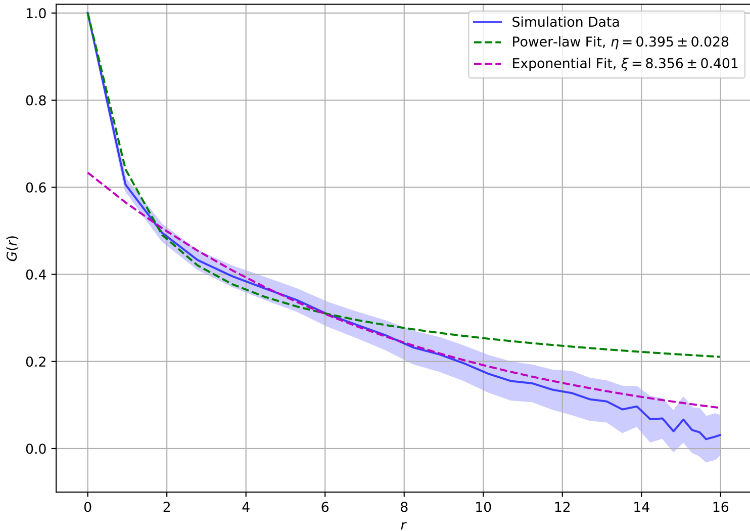
Correlation Function at T = 1.90e - 01 , L = 16
