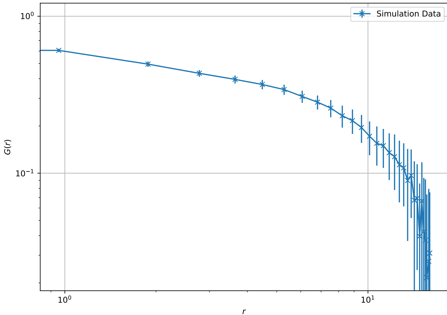
Correlation Function at T = 1.90e - 01 , L = 16 (Log-Log Scale)
