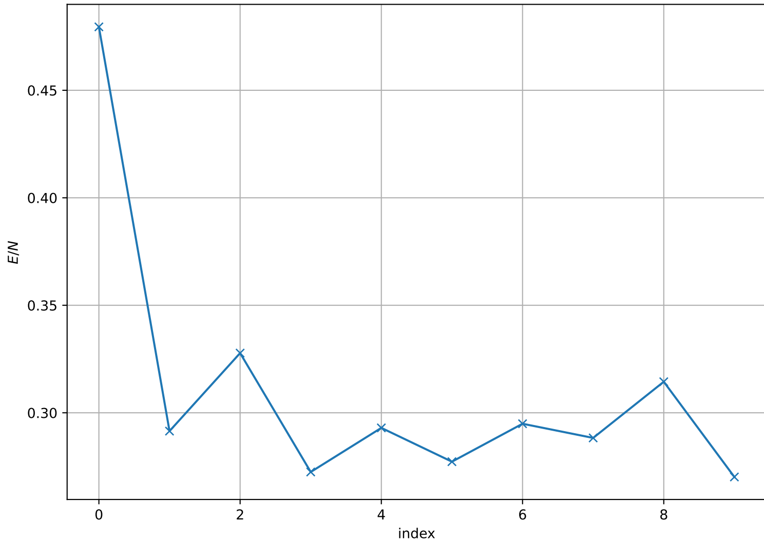
Energy per Site at T = 1.900e - 01 , L = 16
