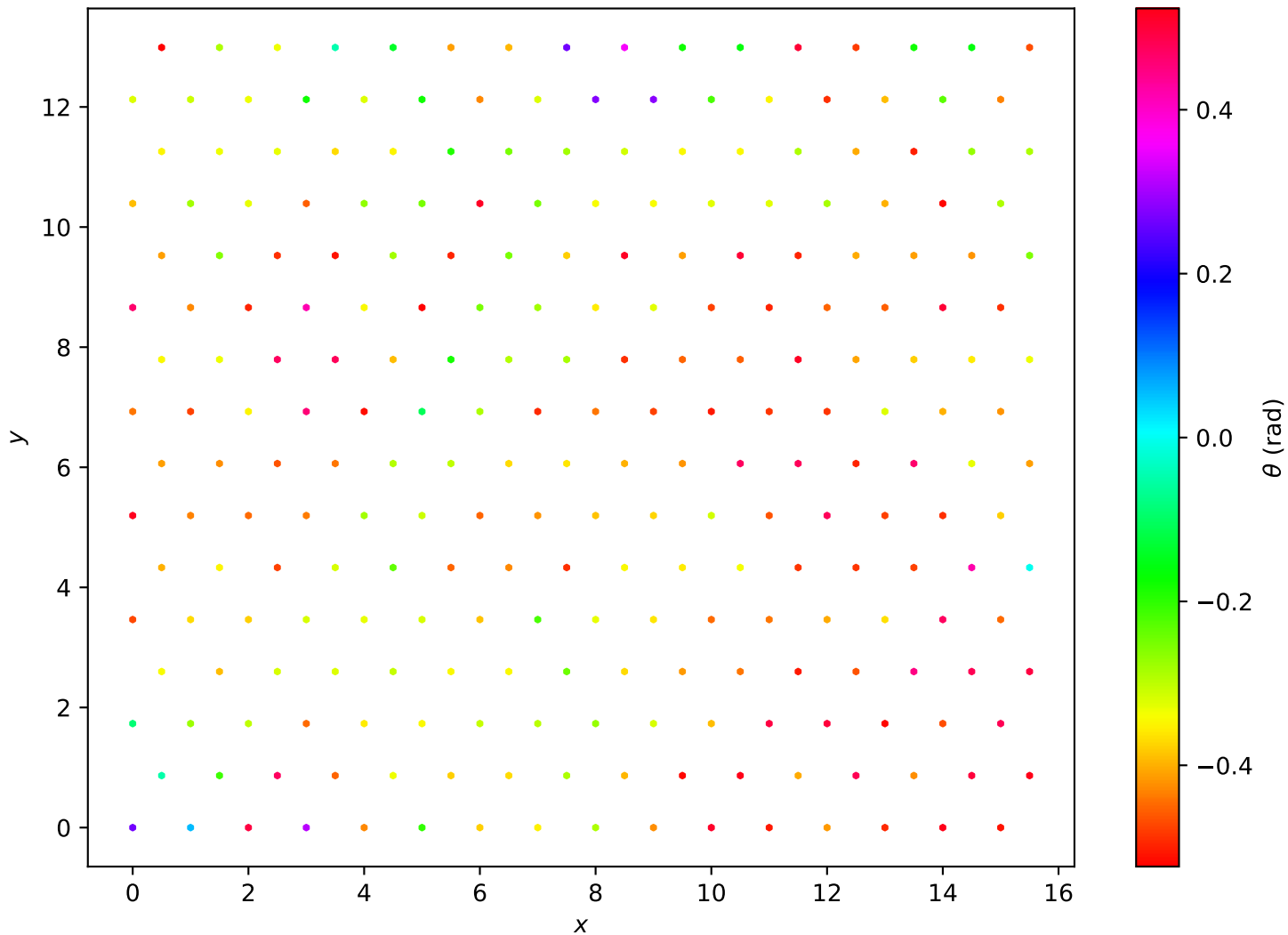
Hexagonal Lattice L=16 , T = 1.90e - 01
