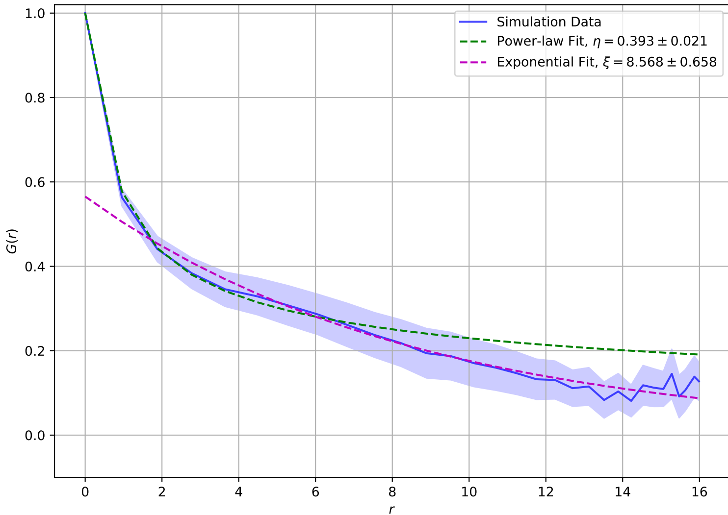
Correlation Function at T = 1.95e - 01 , L = 16
