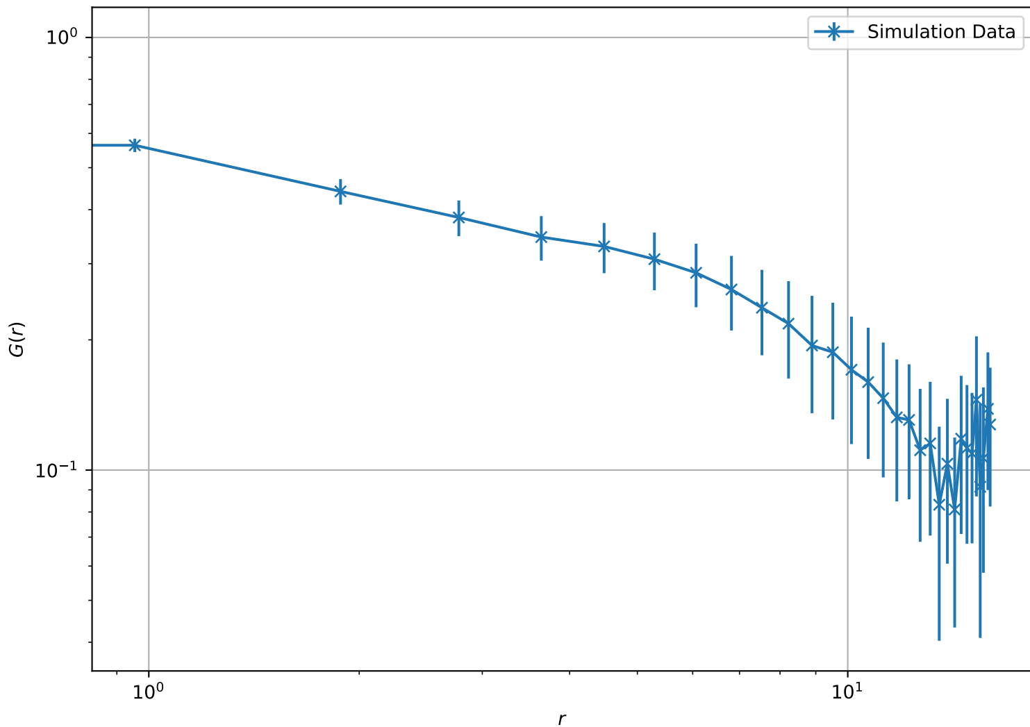
Correlation Function at T = 1.95e - 01 , L = 16 (Log-Log Scale)
