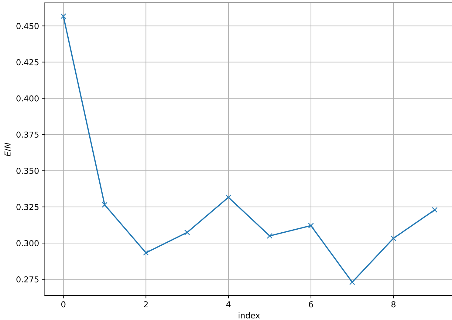
Energy per Site at T = 1.950e - 01 , L = 16
