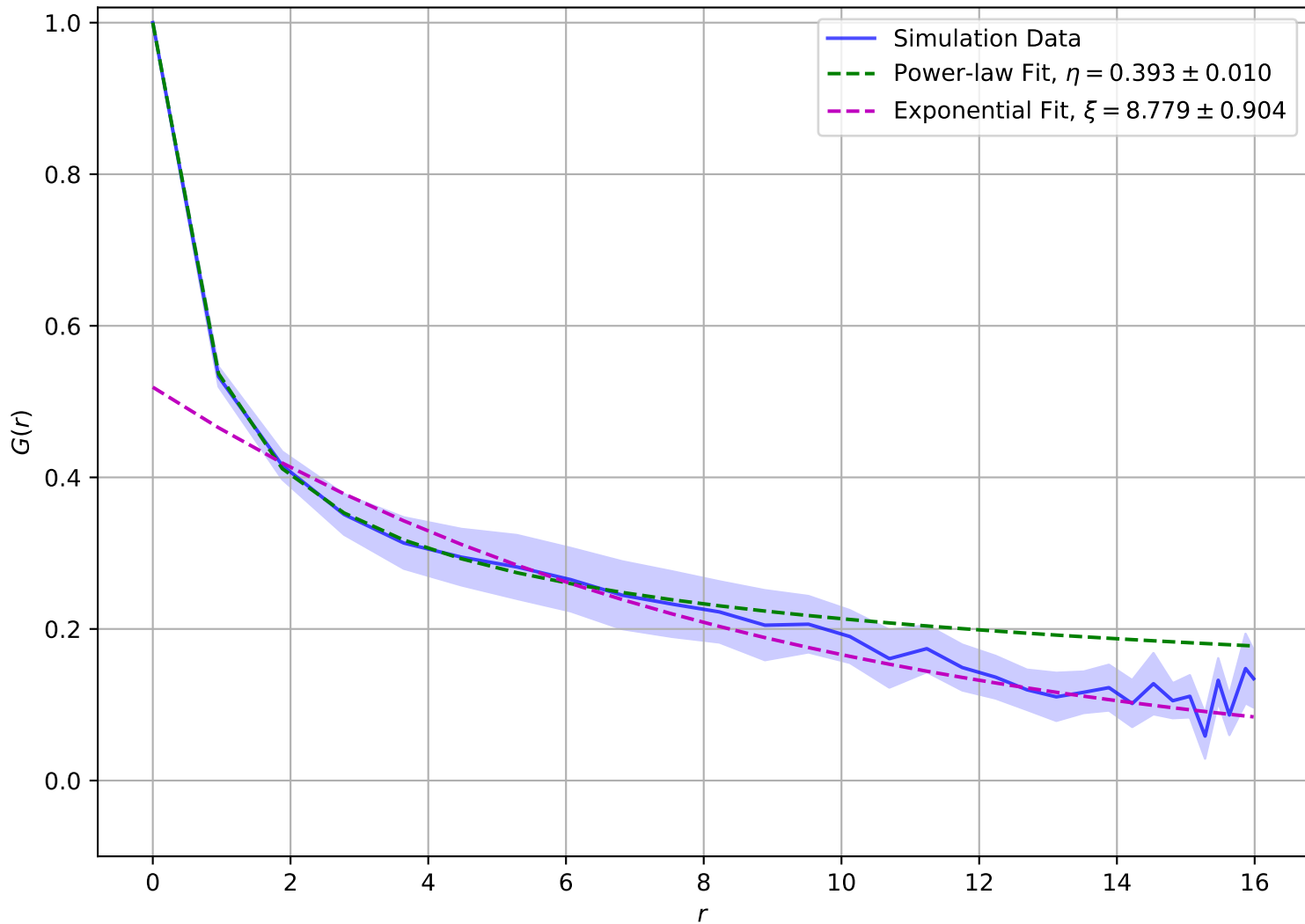
Correlation Function at T = 2.05e - 01 , L = 16
