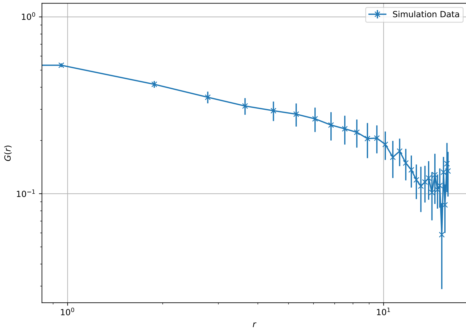
Correlation Function at T = 2.05e - 01 , L = 16 (Log-Log Scale)
