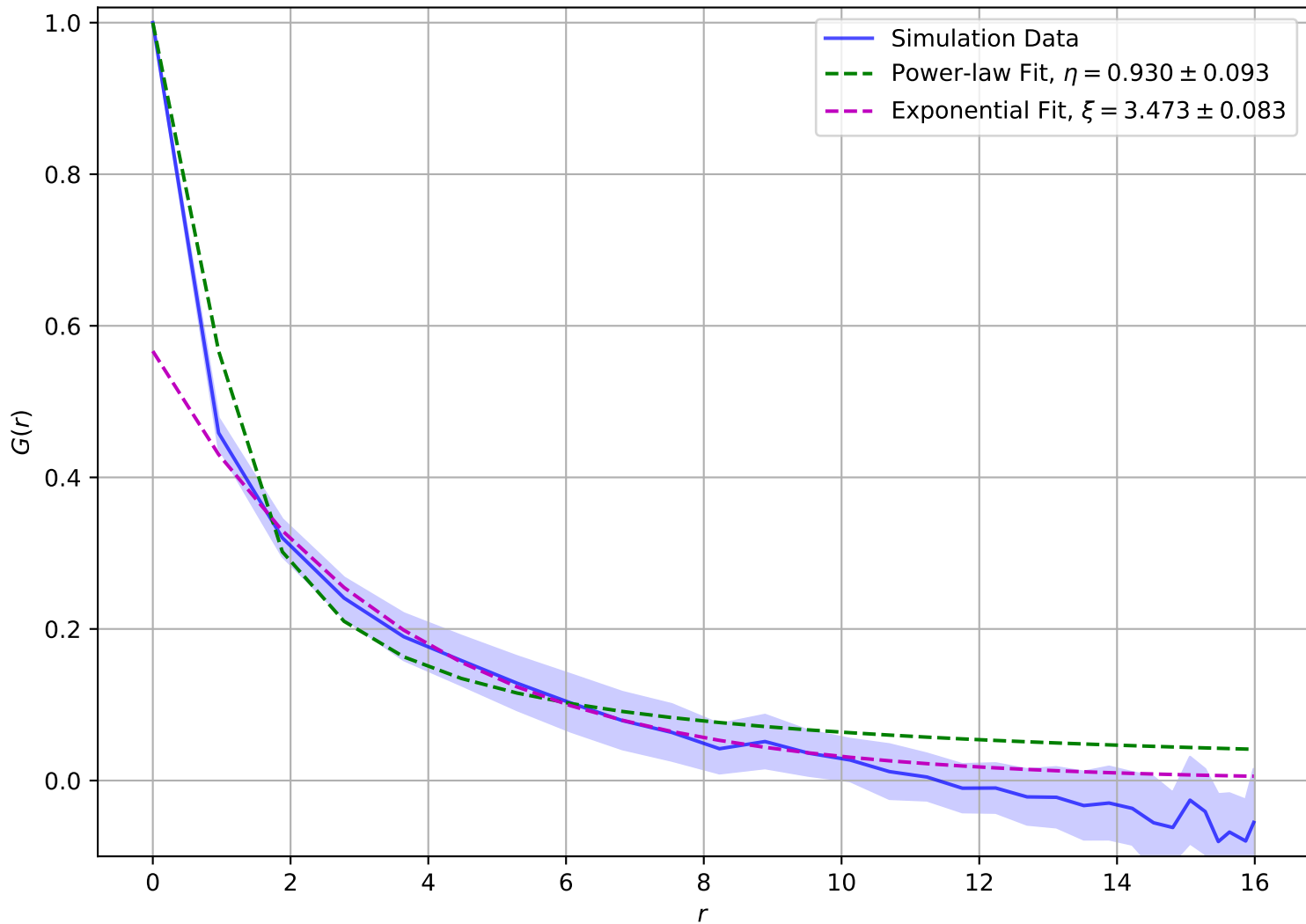
Correlation Function at T = 2.10e - 01 , L = 16
