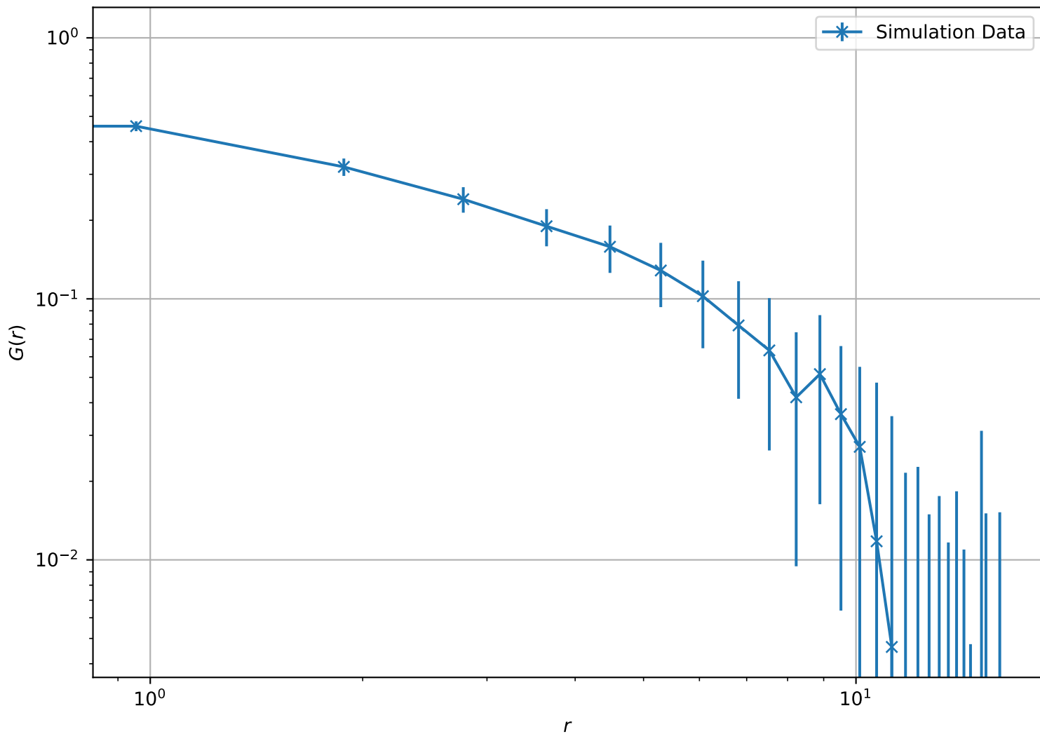
Correlation Function at T = 2.10e - 01 , L = 16 (Log-Log Scale)
