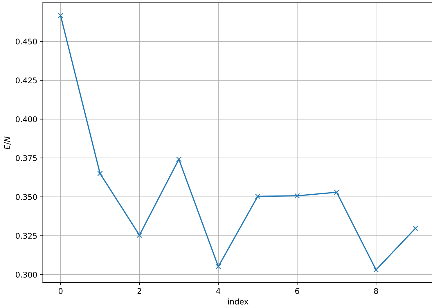
Energy per Site at T = 2.100e - 01 , L = 16
