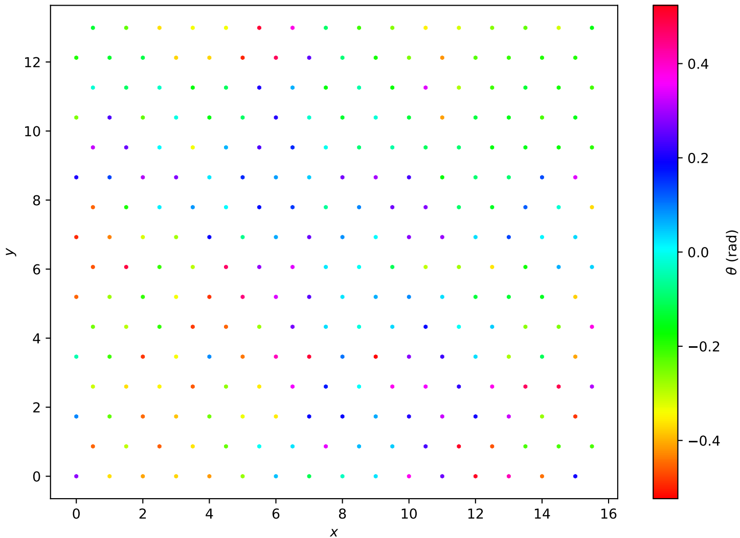
Hexagonal Lattice L=16 , T = 2.10e - 01
