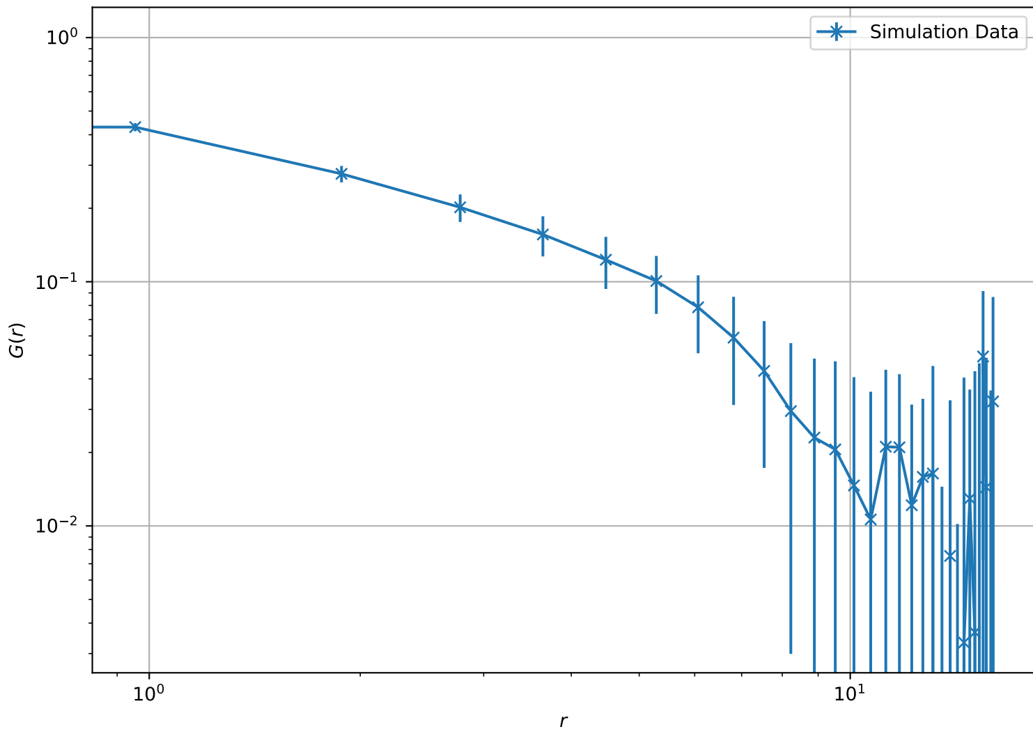
Correlation Function at T = 2.15e - 01 , L = 16 (Log-Log Scale)
