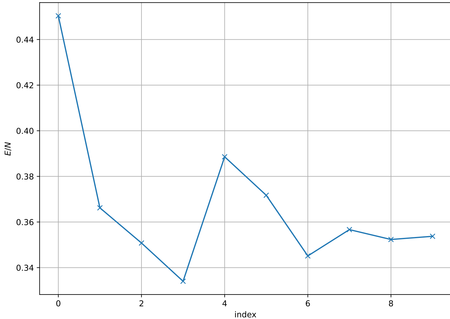
Energy per Site at T = 2.150e - 01 , L = 16
