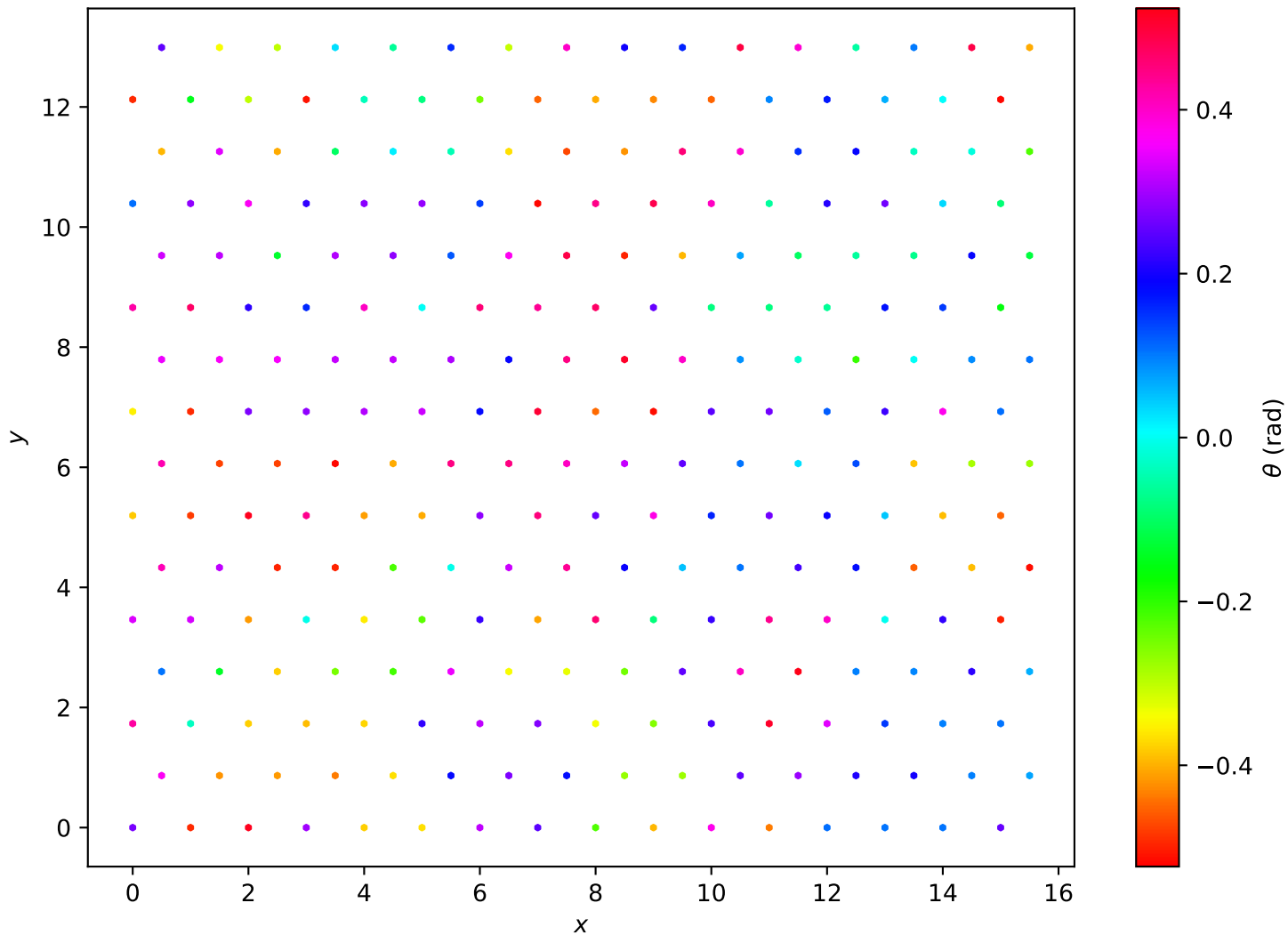
Hexagonal Lattice L=16 , T = 2.15e - 01
