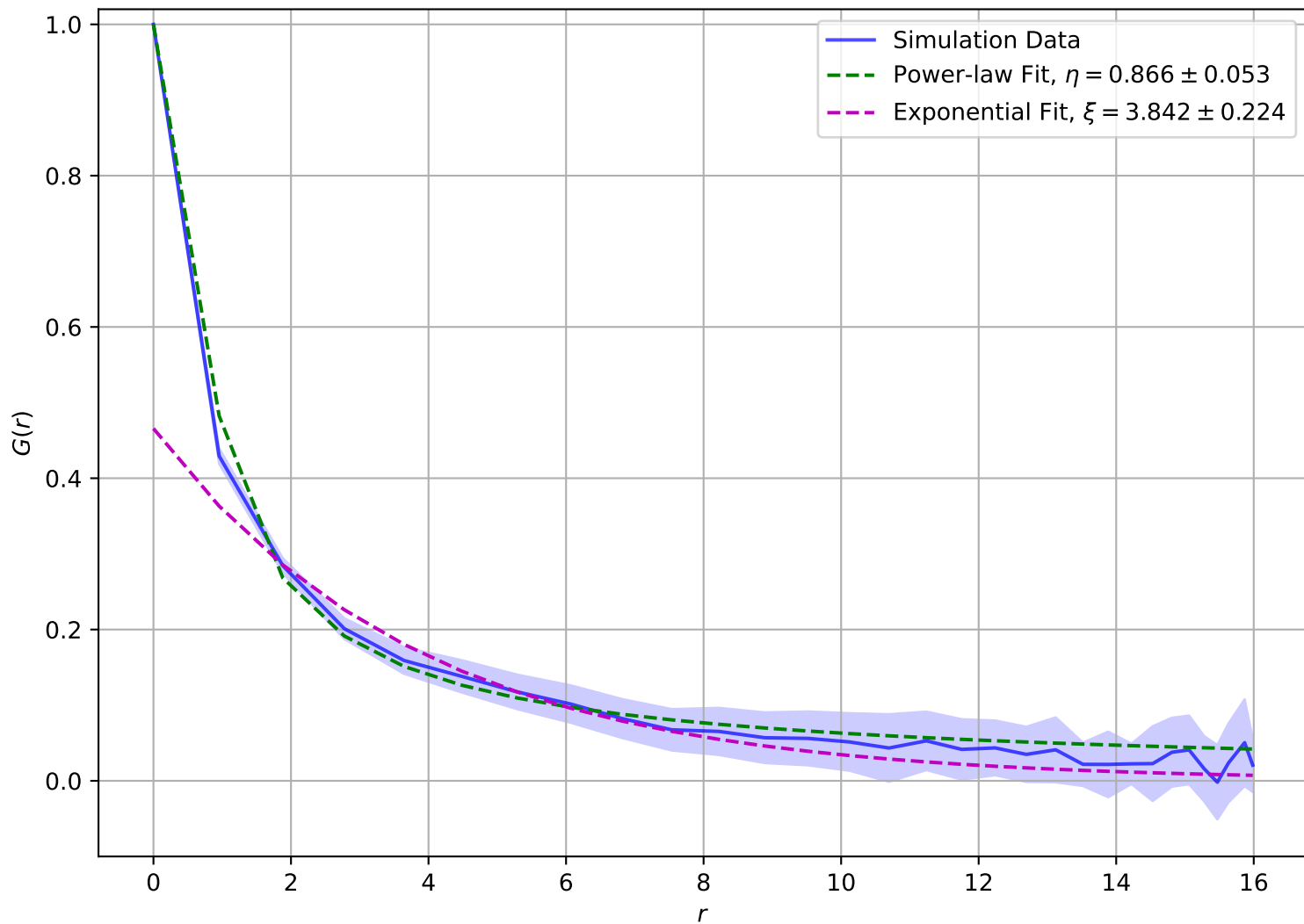
Correlation Function at T = 2.20e - 01 , L = 16
