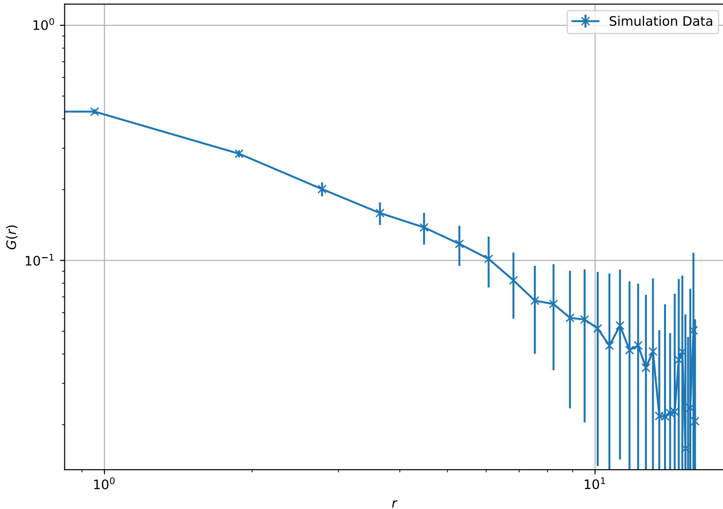
Correlation Function at T = 2.20e - 01 , L = 16 (Log-Log Scale)
