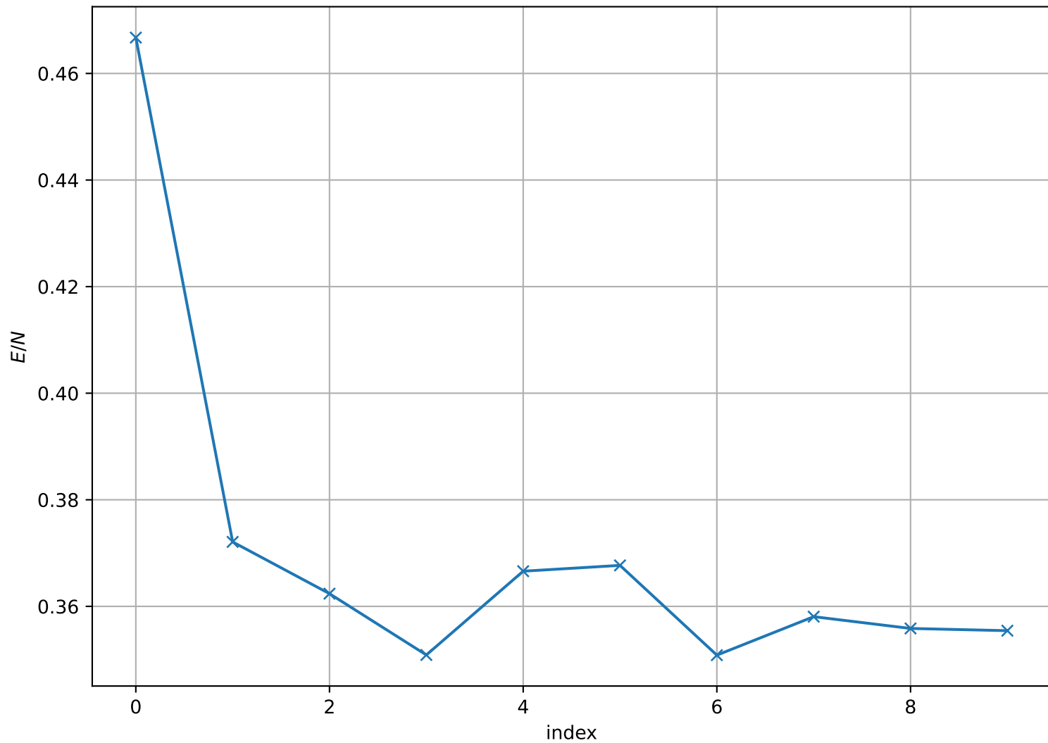
Energy per Site at T = 2.200e - 01 , L = 16
