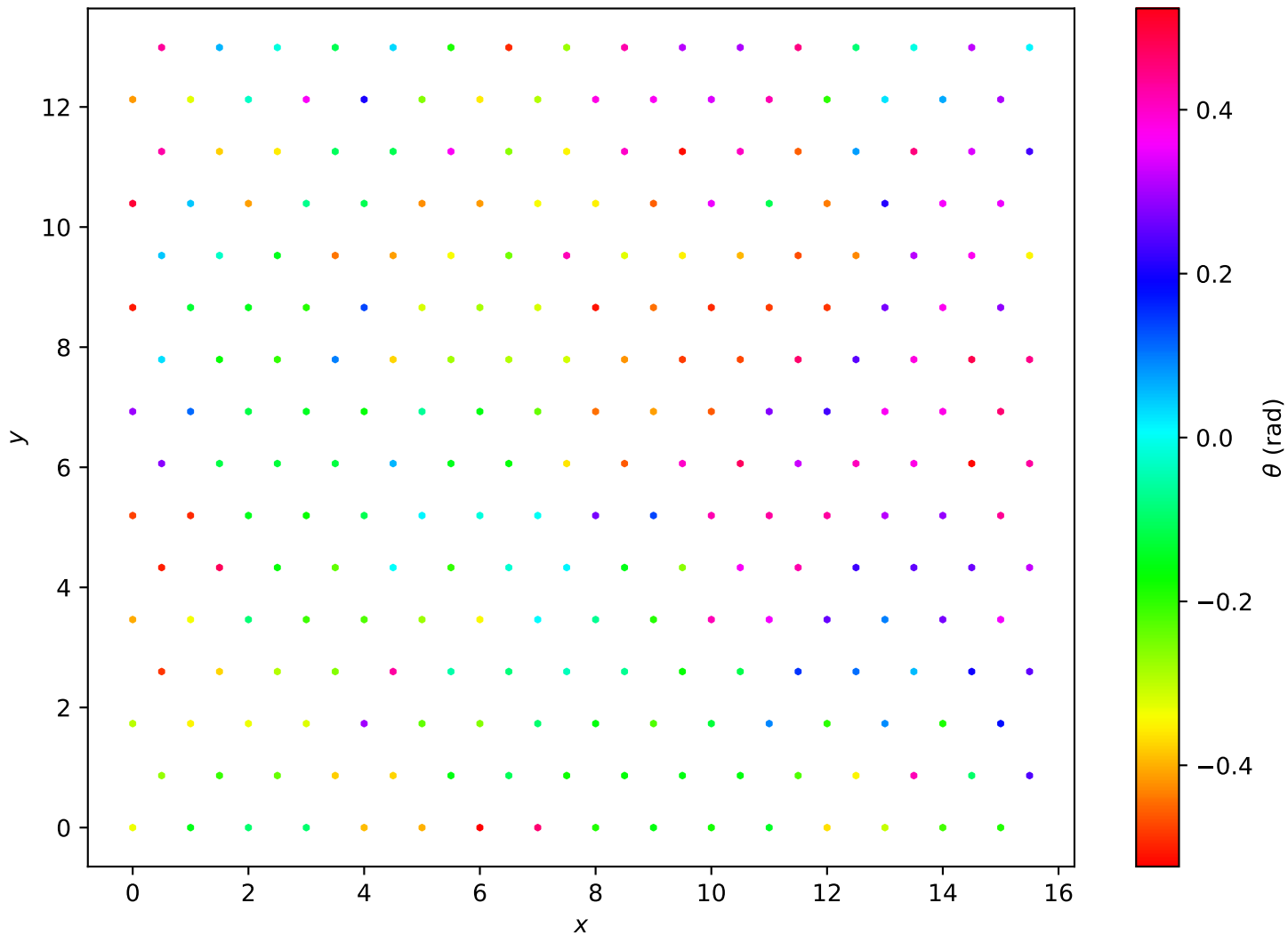
Hexagonal Lattice L=16 , T = 2.20e - 01
