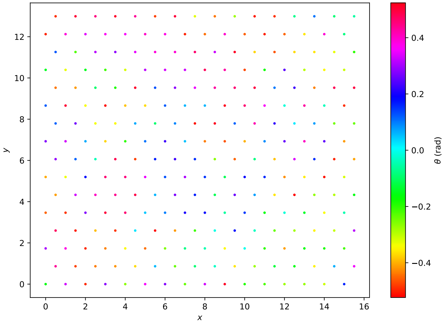
Hexagonal Lattice L=16 , T = 2.50e - 01
