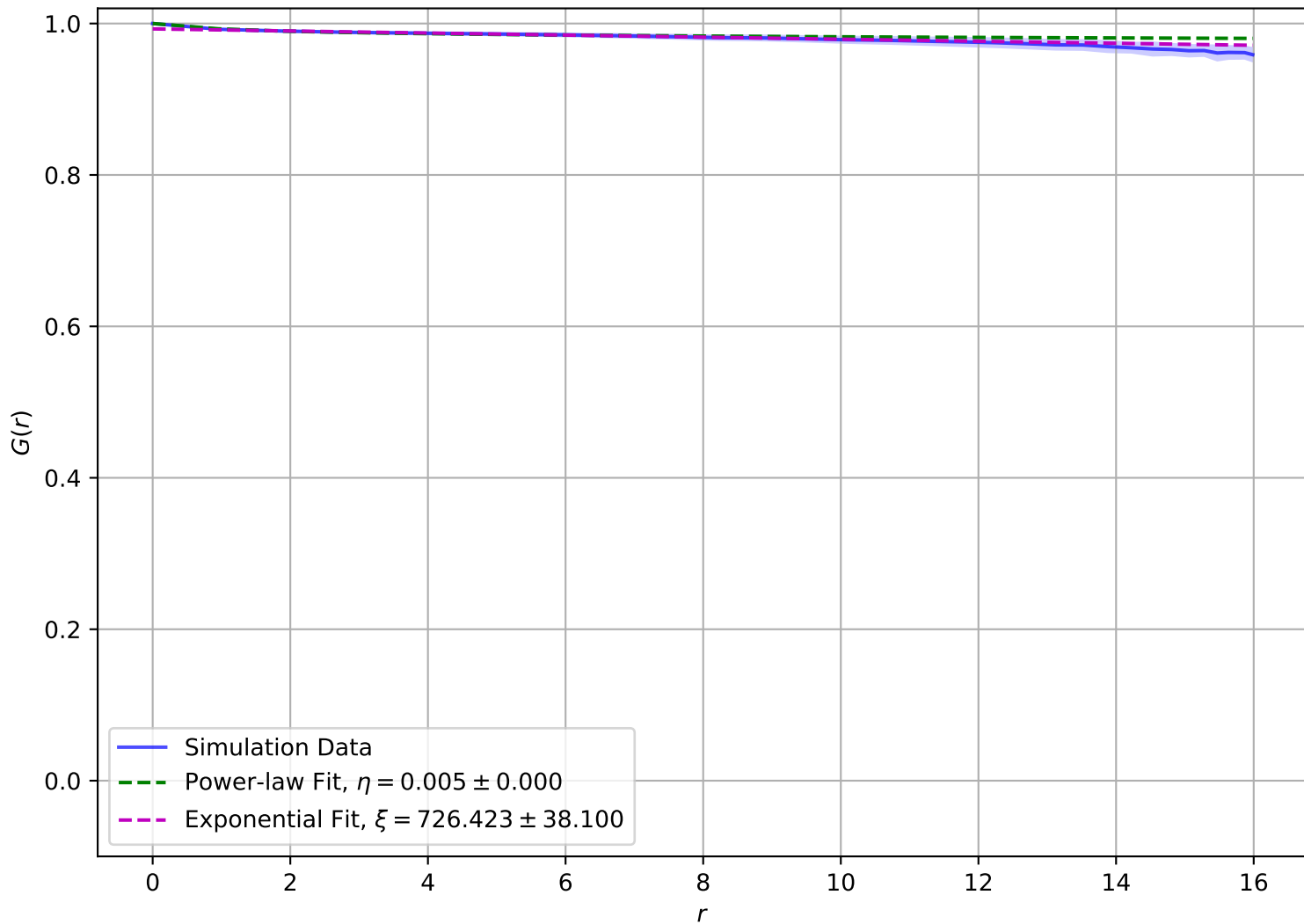
Correlation Function at T = 5.00e - 02 , L = 16
