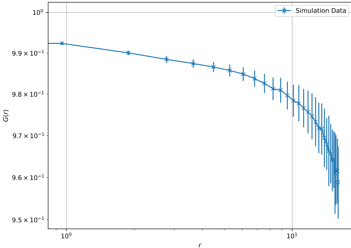
Correlation Function at T = 5.00e - 02 , L = 16 (Log-Log Scale)
