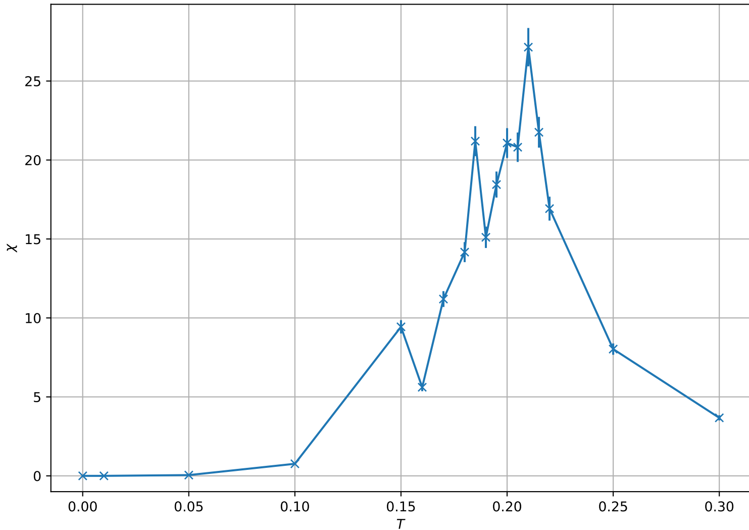
Susceptibility \chi vs Temperature for L = 16
