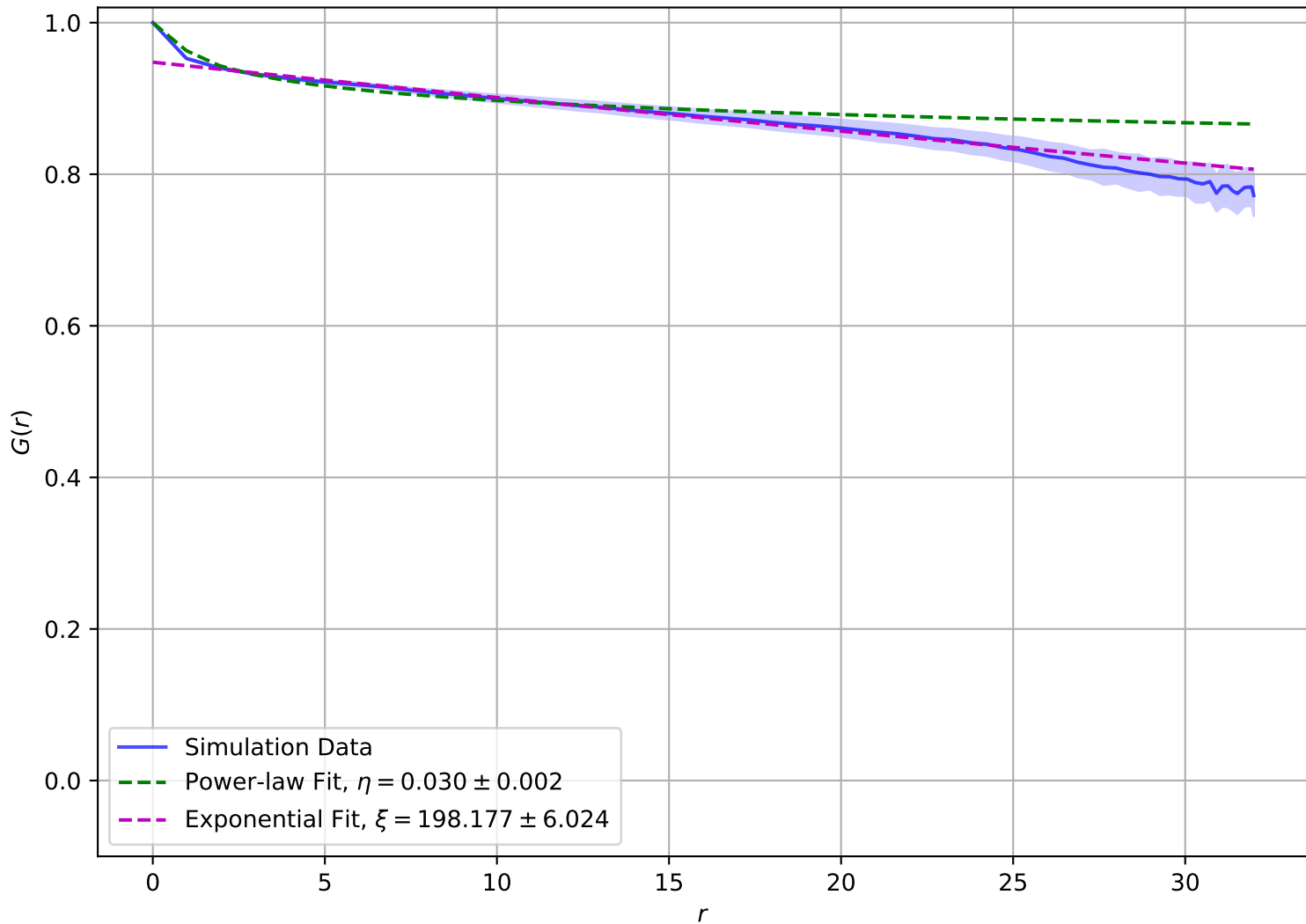
Correlation Function at T = 1.00e - 01 , L = 32
