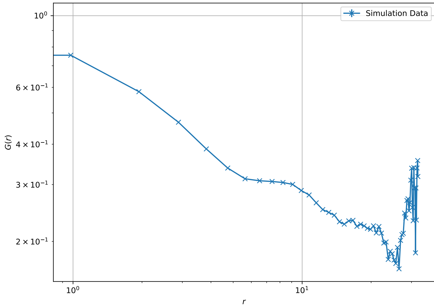
Correlation Function at T = 1.00\text{e} - 05 , L = 32 (Log-Log Scale)
