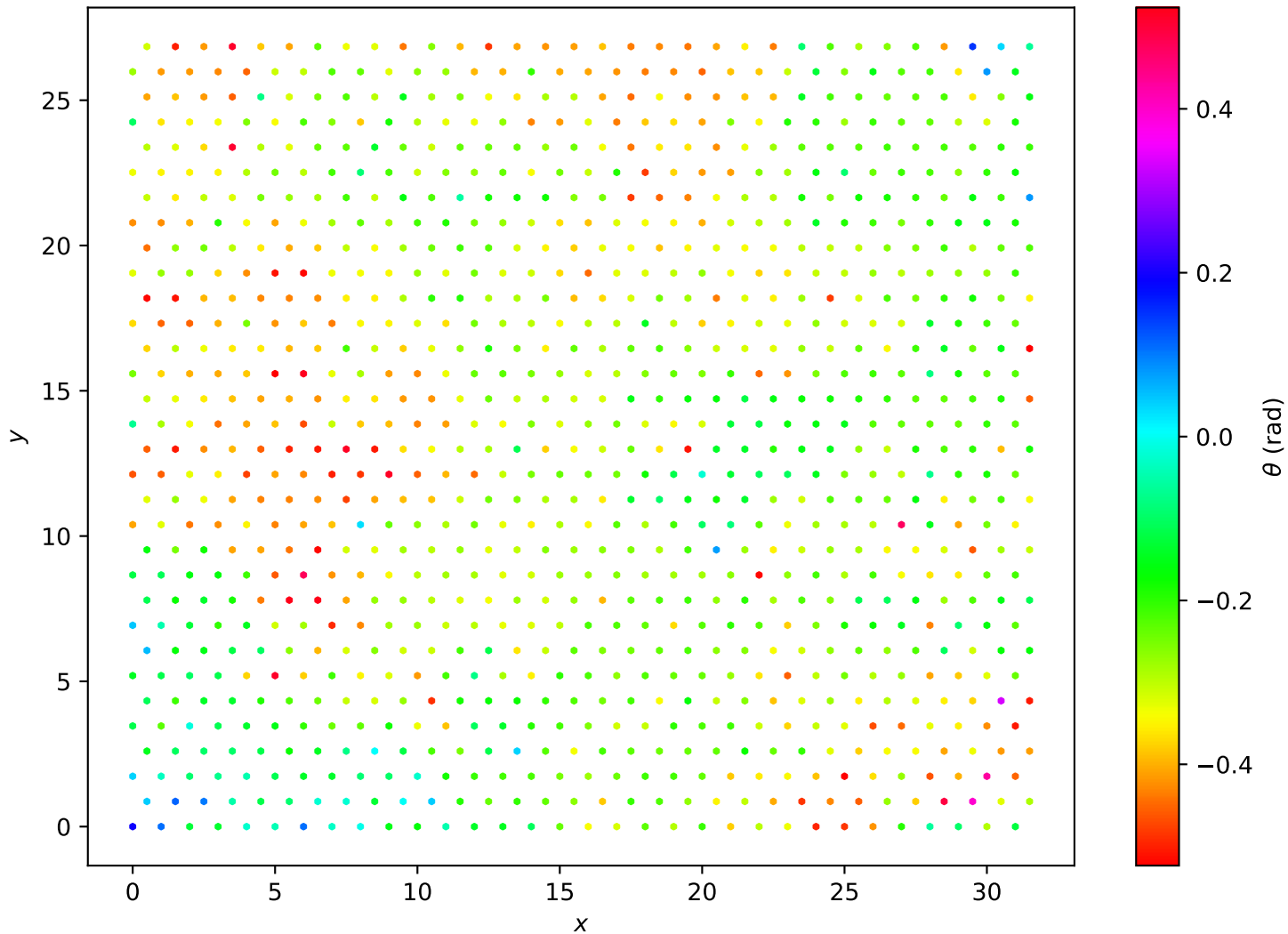
Hexagonal Lattice L=32 , T = 1.60e - 01
