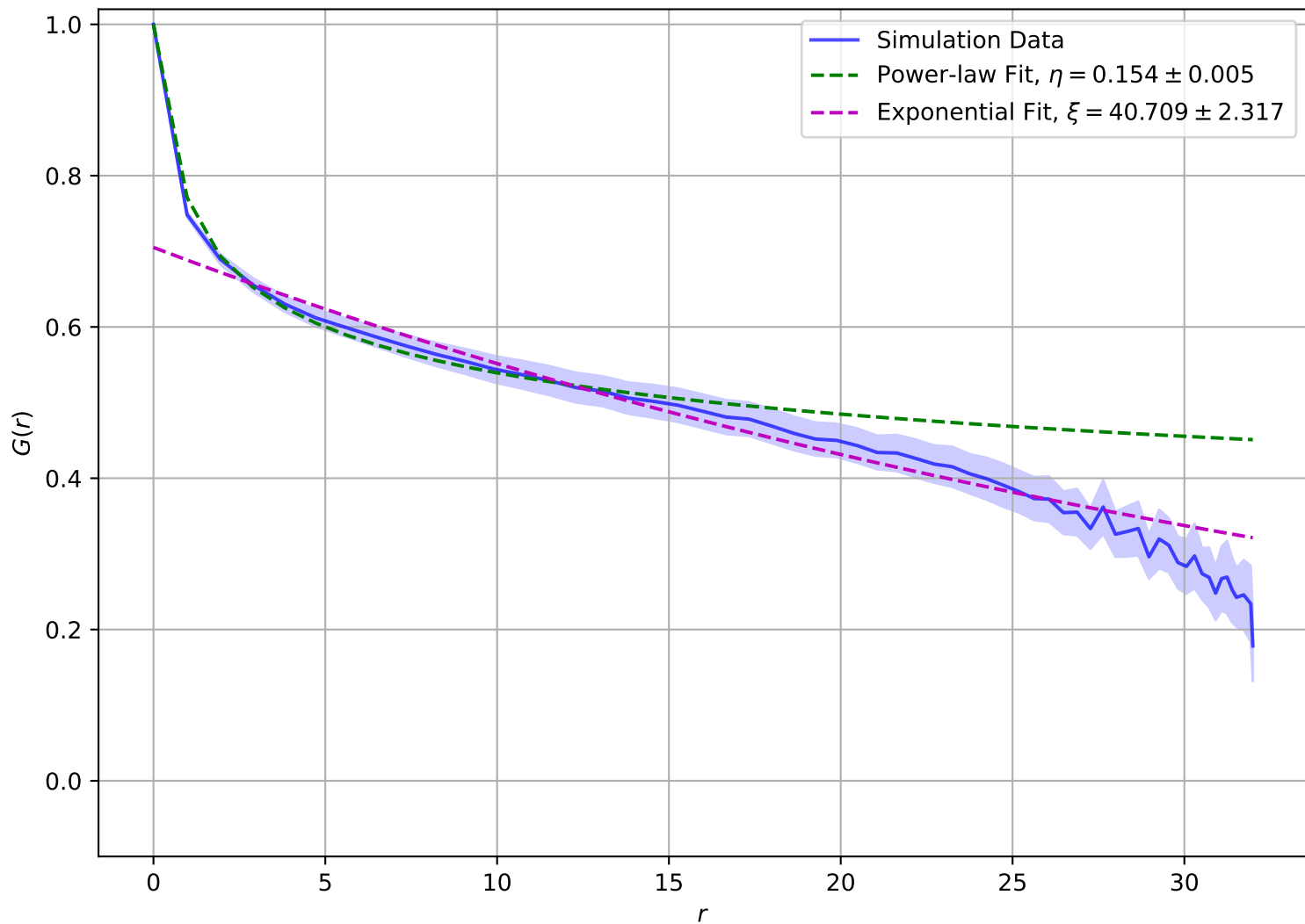
Correlation Function at T = 1.70e - 01 , L = 32
