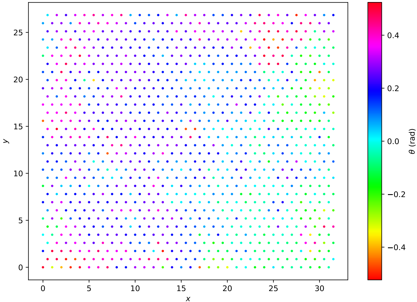
Hexagonal Lattice L=32 , T = 1.70e - 01
