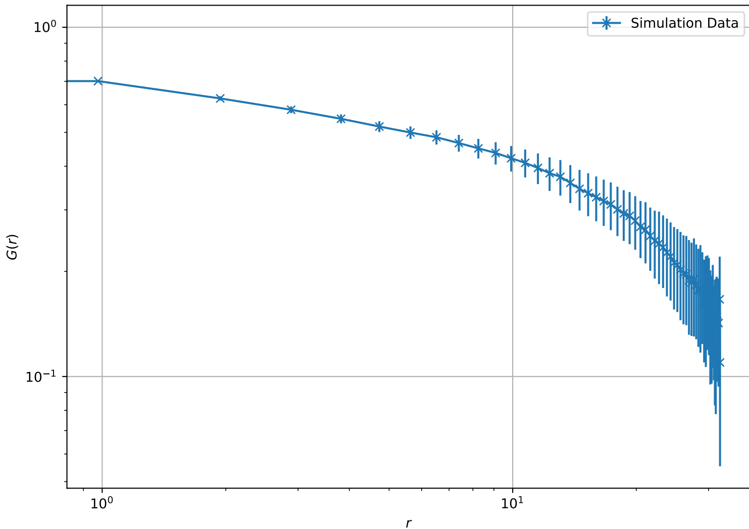
Correlation Function at T = 1.80e - 01 , L = 32 (Log-Log Scale)
